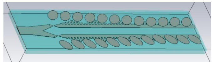
Fig. 4: Three-dimensional perspective view of the full antenna structure showing the layered stack comprising the metal background, the lower dielectric substrate carrying the SSPP transmission lines, the air gap (thickness t_1 ), the upper dielectric substrate (thickness t_2 ) carrying the elliptical patches, and the overall physical extent of the antenna.
