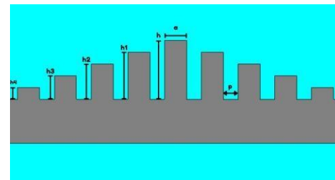
Fig. 3: Side profile of the SSPP transmission line unit cell, illustrating the key geometric parameters: groove height h , groove width a , and unit-cell period p . The stepped groove profile that produces the tapered dispersion characteristic is also visible.
