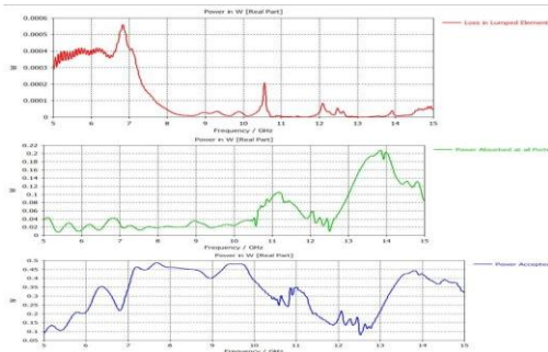
Fig. 13: Simulated power budget for Mode 1 showing the loss in lumped elements (red), power absorbed at all ports (green), and power accepted (blue) as functions of frequency. The diode loss is concentrated below 8 GHz and becomes negligible within the target operating band.
