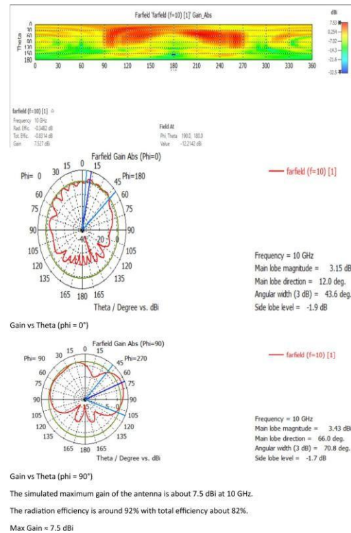
Fig. 10: Simulated gain versus angle at 10 GHz for both principal planes (Mode 1). Main lobe magnitude in the \phi = 0^\circ plane: 3.15 dBi at \theta = 12^\circ ; angular width (3 dB): 43.6°; side-lobe level: -1.9 dB. Main lobe magnitude in the \phi = 90^\circ plane: 3.43 dBi at \theta = 66^\circ ; angular width (3 dB): 70.8°; side-lobe level: -1.7 dB.
