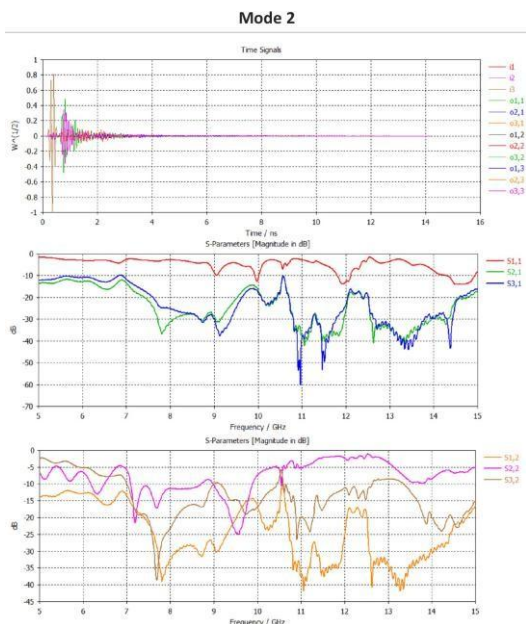
(b) Mode 2 S-parameters over 5–15 GHz.
