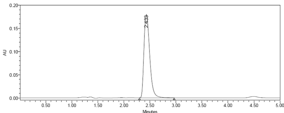
Figure 2: typical chromatogram of by proposed method
