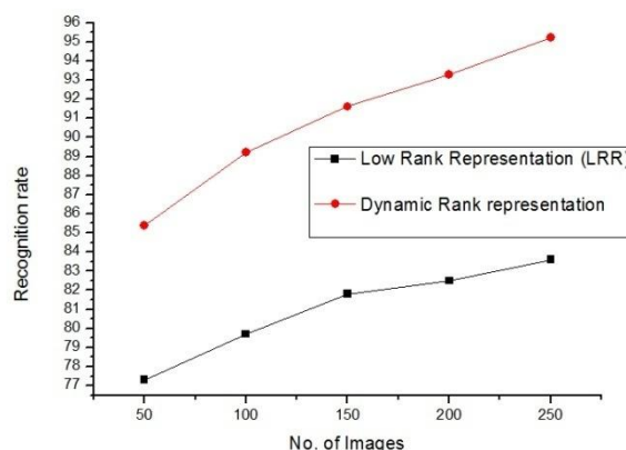
Figure 7 Comparison between low-rank and dynamic rank representation
