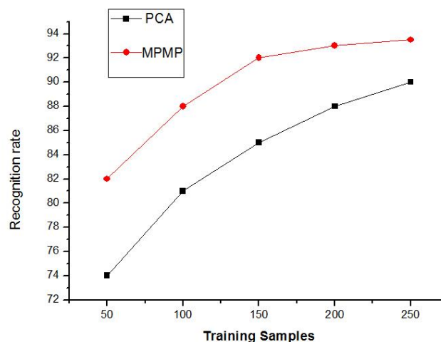
Figure 4 Recognition rate of Multi-Partition Max Pooling (MPMP)
