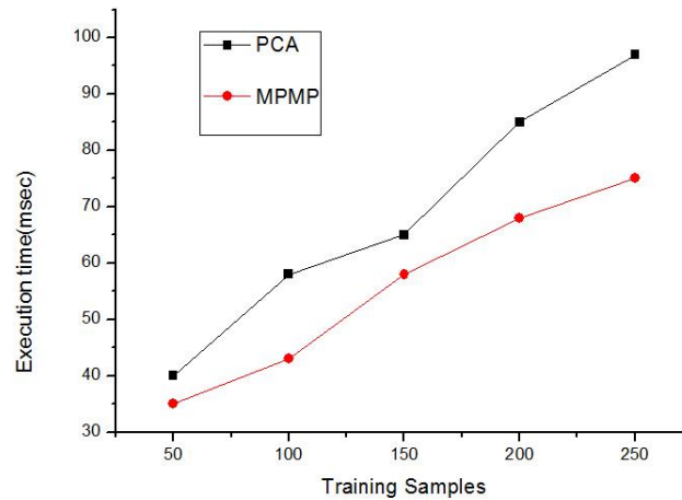
Figure 5 Execution time of Multi-Partition Max Pooling (MPMP)
